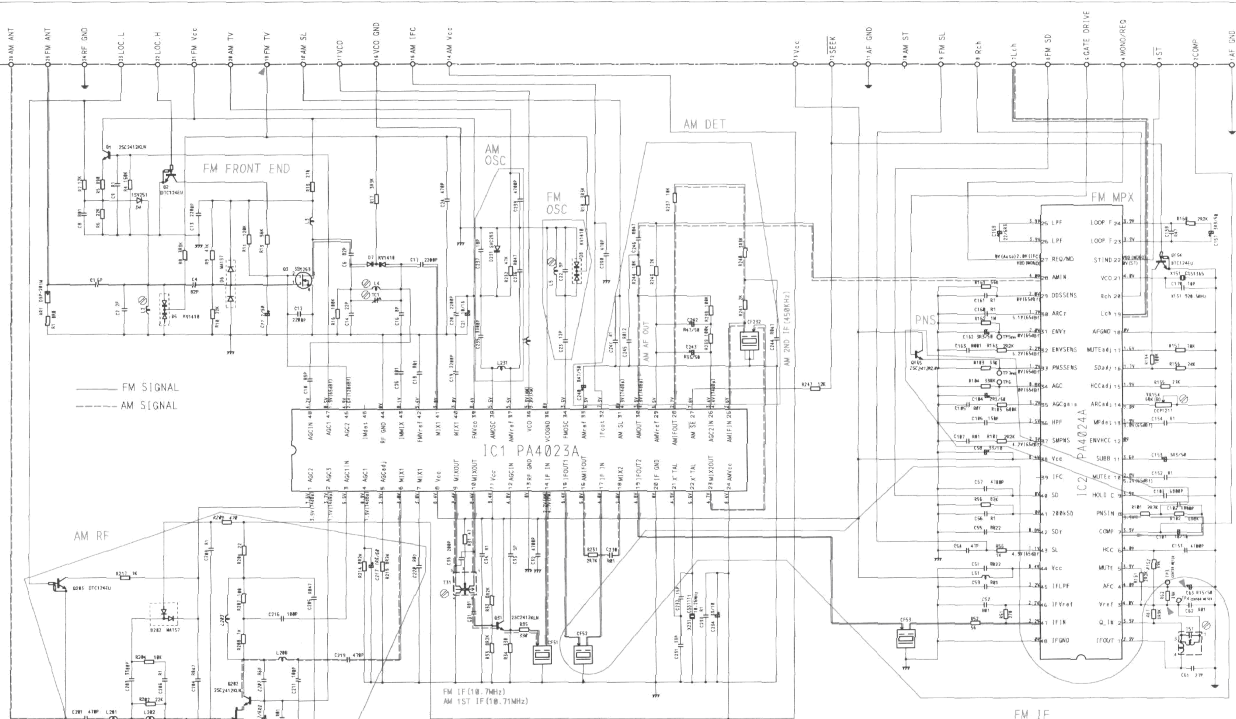
Схема автомагнитолы PIONEER KEH-1100, KEH-1150, KEH-1300, KEH-1300SDK, KEH-1311, KEH-1400, KEH-1450
