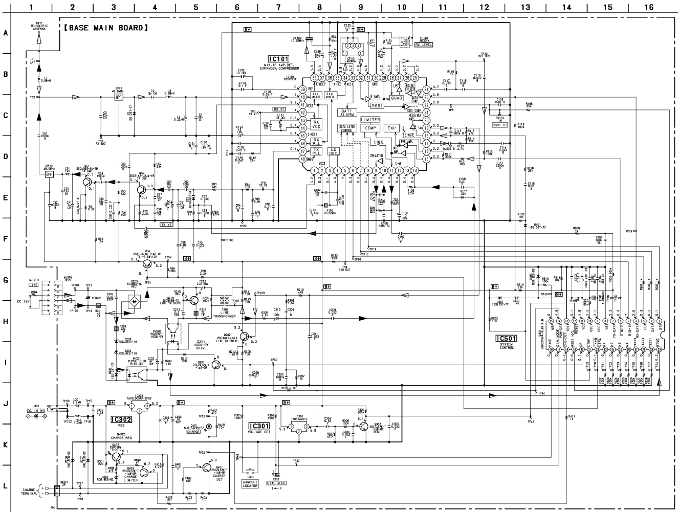
5-5. SCHEMATIC DIAGRAM — BASE UNIT SECTION —
