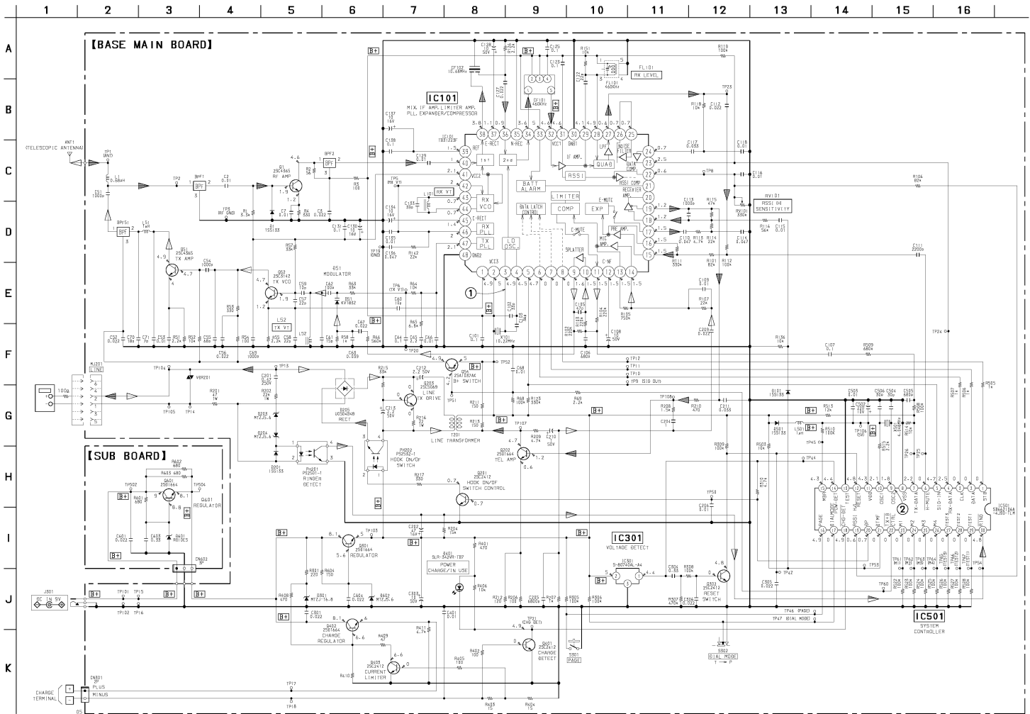
6-5. SCHEMATIC DIAGRAM – BASE UNIT Section – • See page 24 for Waveforms.
