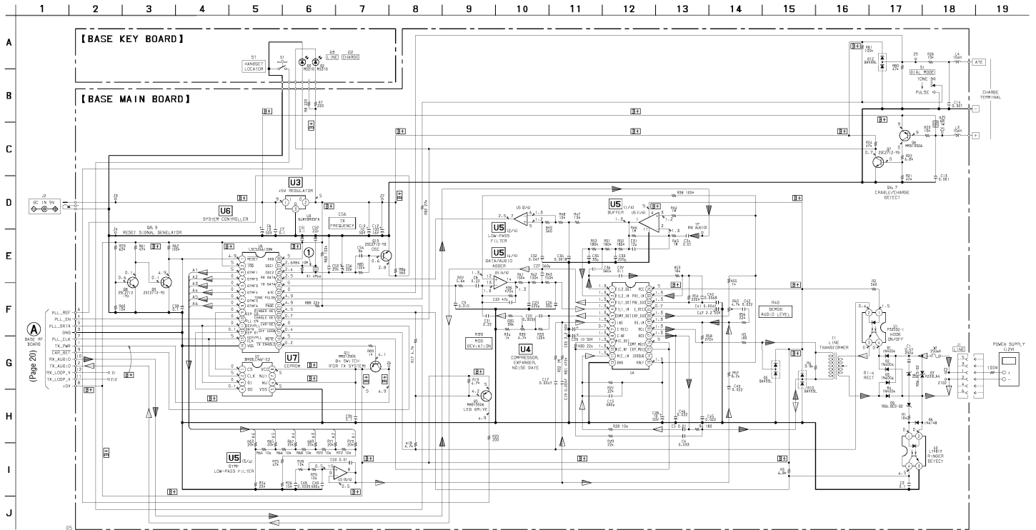
5-6. SCHEMATIC DIAGRAM – BASE MAIN/BASE KEY Boards – • See page 16 for Waveform. • See page 30 for IC Block Diagrams.
