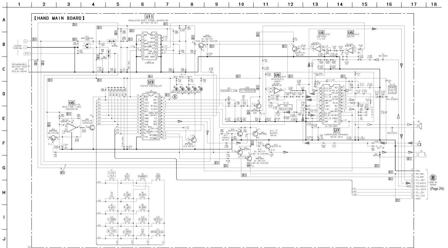
5-8. SCHEMATIC DIAGRAM – HAND MAIN Board – • See page 16 for Waveform. • See page 30 for IC Block Diagrams.
