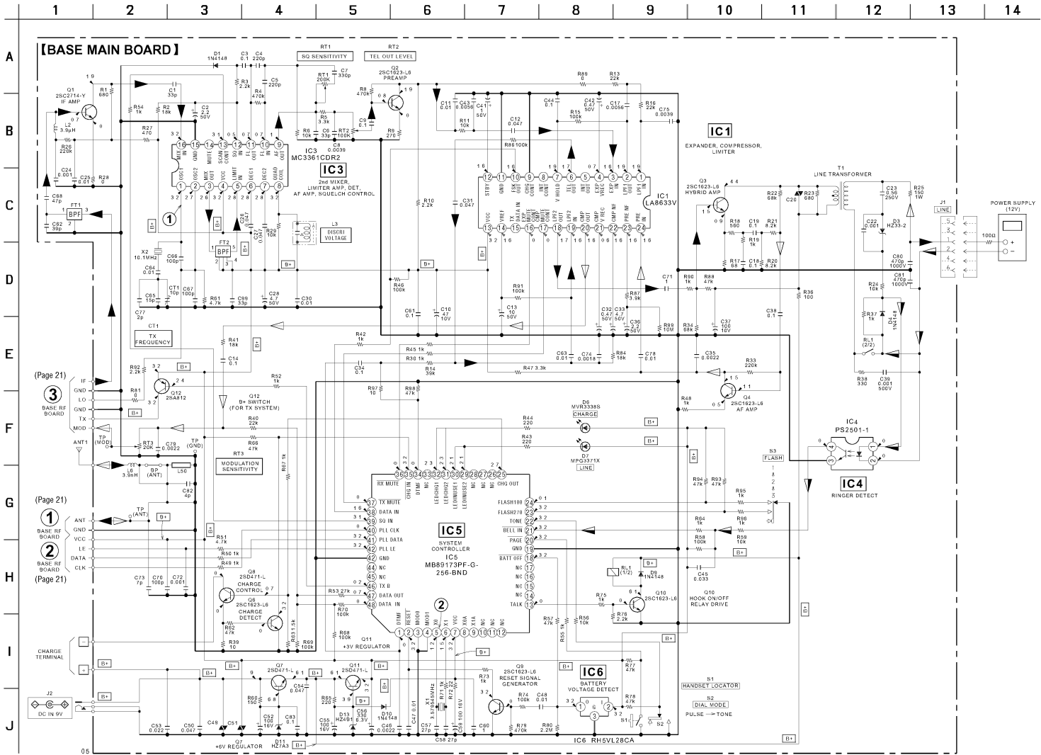
5-7. SCHEMATIC DIAGRAM – BASE MAIN Section – • See page 24 for Waveforms. • See page 28 for IC Block Diagrams.
