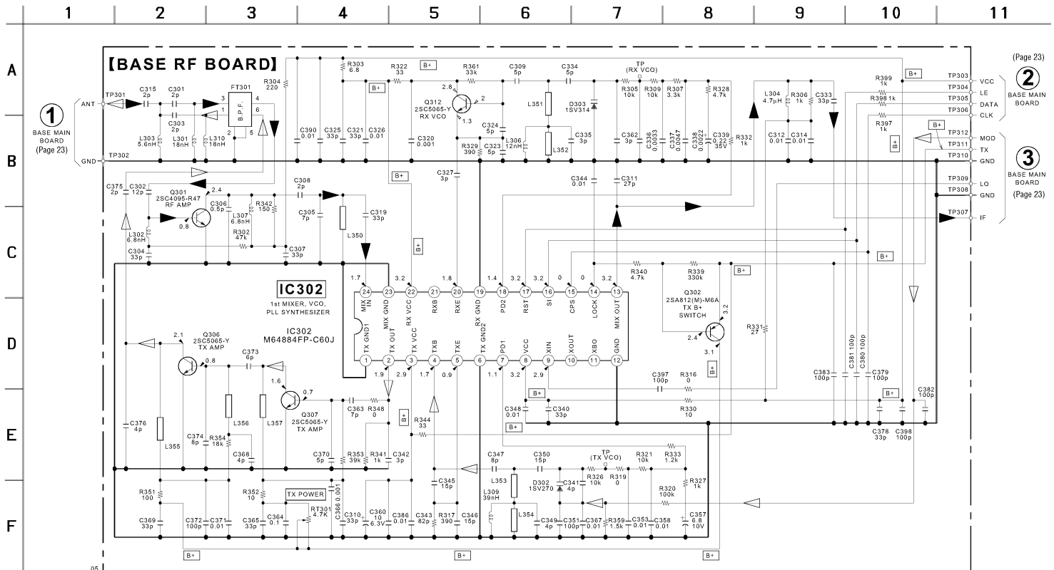
5-5. SCHEMATIC DIAGRAM – BASE RF Section – • See page 28 for IC Block Diagram.
