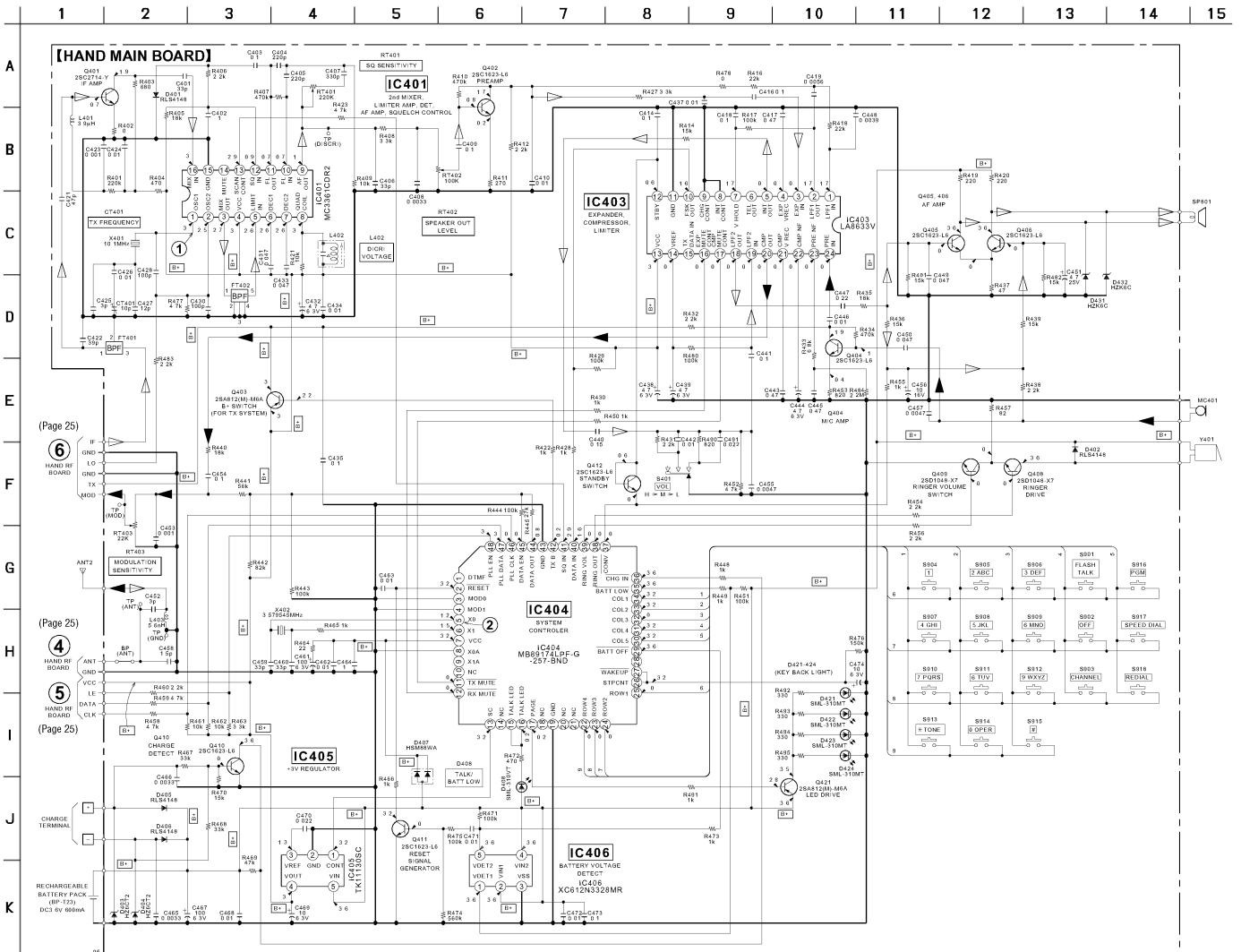
5-11. SCHEMATIC DIAGRAM – HAND MAIN Section – • See page 24 for Waveforms. • See page 28 for IC Block Diagrams.
