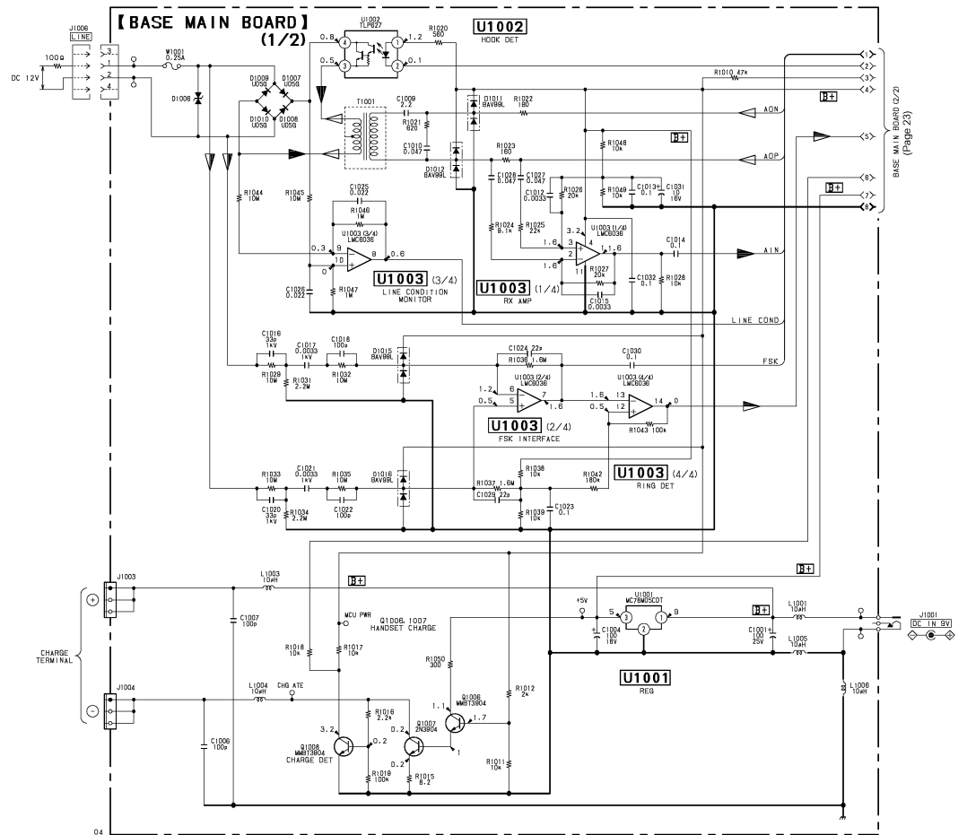
SCHEMATIC DIAGRAM — BASE UNIT SECTION (1/2) —
