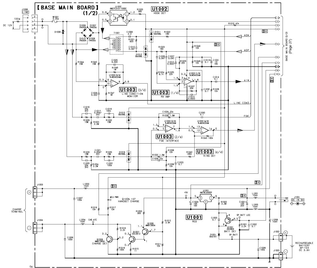
SCHEMATIC DIAGRAM — BASE MAIN SECTION (1/2) —
