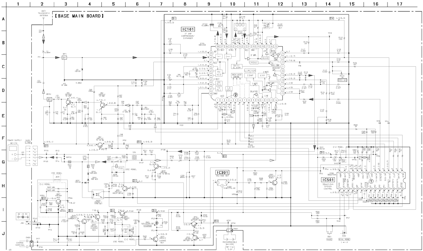
5-3. SCHEMATIC DIAGRAM – BASE UNIT SECTION – • See page 20 for Waveforms.
