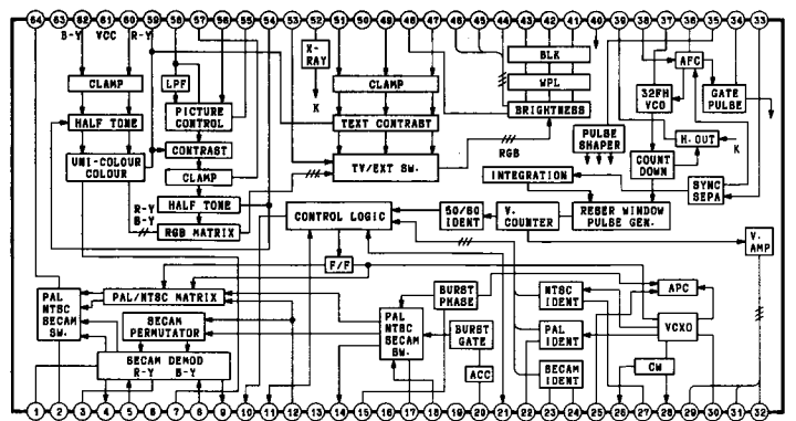
BLOCK DIAGRAM FOR IC601 (TA8653N)
